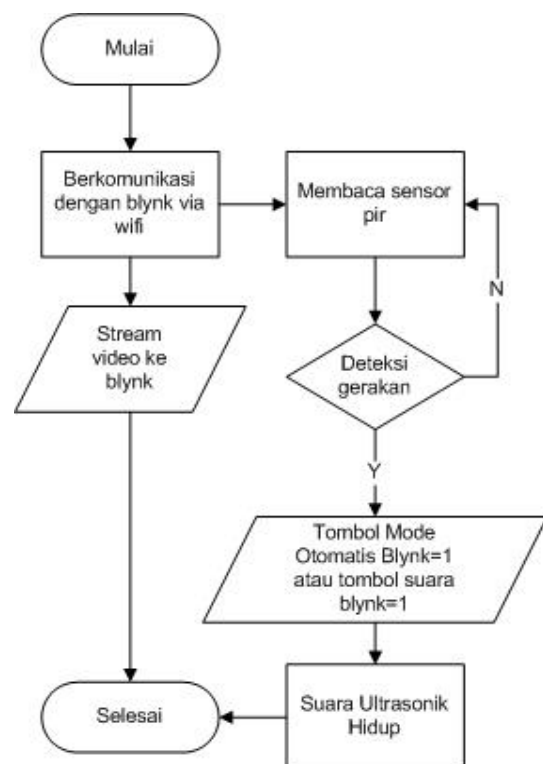
Gambar 1. Flowchart Penelitian
